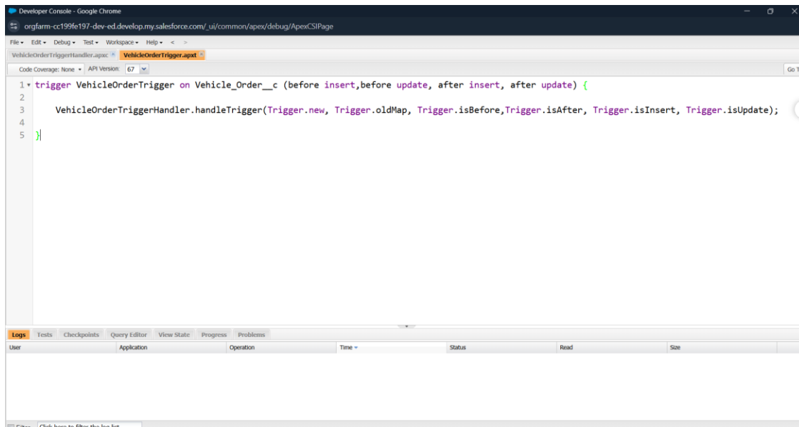
Figure 4.2: VehicleOrderTrigger Apex trigger definition, showing the single delegating call into VehicleOrderTriggerHandler.
