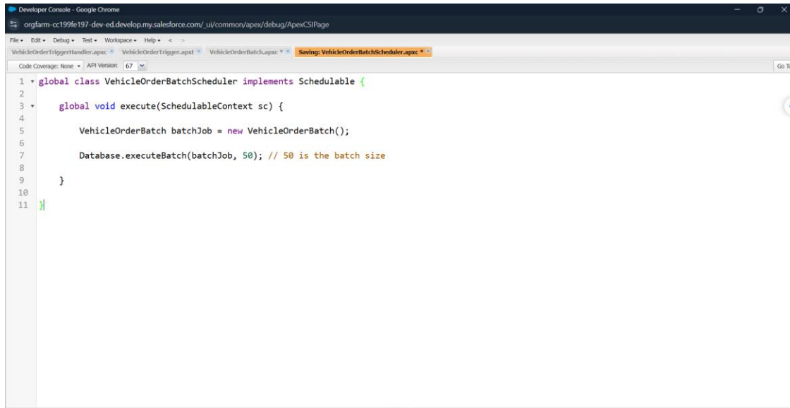
Figure 4.4: VehicleOrderBatchScheduler Apex class implementing Schedulable, executing VehicleOrderBatch with a batch size of 50.
