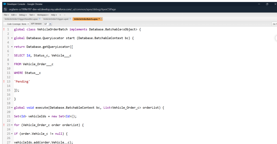
Figure 4.3: VehicleOrderBatch Apex class implementing Database.Batchable<sObject>, showing the start() method's QueryLocator selecting Pending Vehicle Order records.
