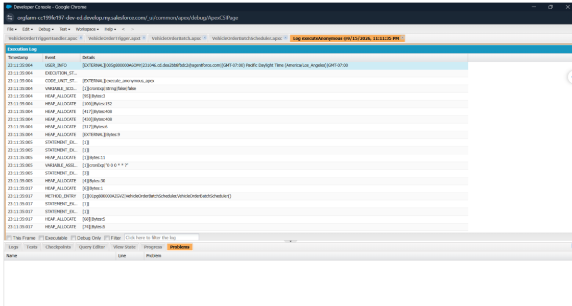
Figure 4.6: Developer Console execution log for the System.schedule() call, showing METHOD_ENTRY into VehicleOrderBatchScheduler with zero problems reported.
