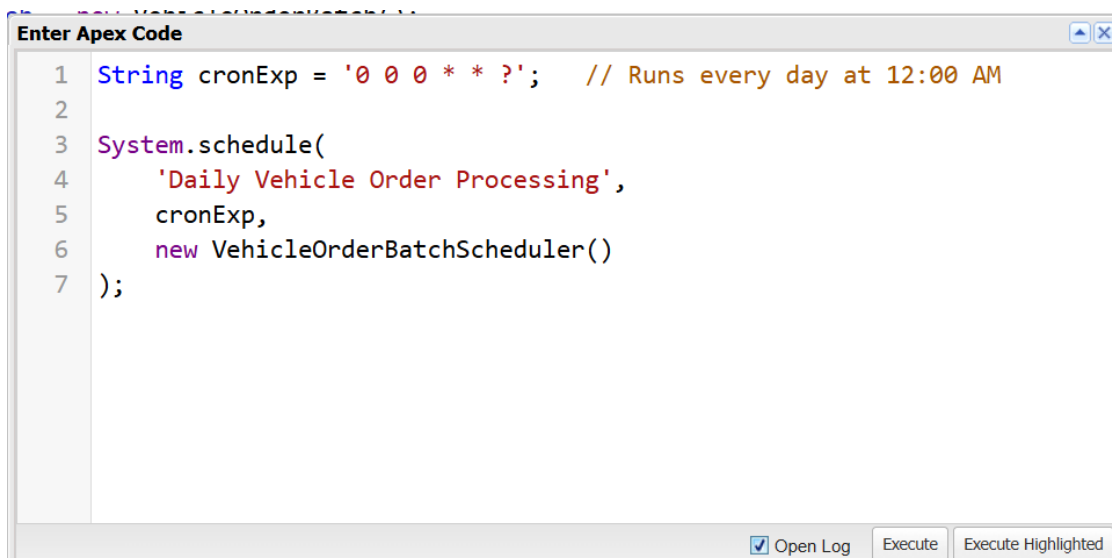
Figure 4.5: Execute Anonymous Apex window used to schedule the VehicleOrderBatchScheduler job with System.schedule() and a daily CRON expression.
