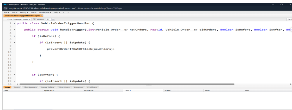
Figure 4.1: VehicleOrderTriggerHandler Apex class opened in the Developer Console, showing the handleTrigger method routing before/after insert and update contexts to preventOrderIfOutOfStock .
