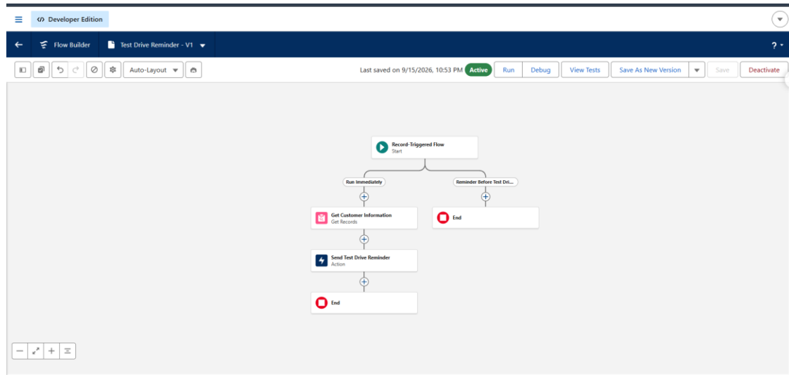
Figure 2.20: Flow Builder canvas for the 'Test Drive Reminder' Record-Triggered Flow, showing the immediate path (Get Customer Information → Send Test Drive Reminder) and the Scheduled Path branch.
